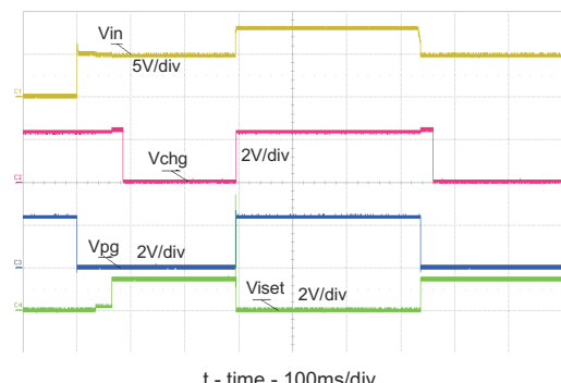
Figure 9-7. OVP from Normal Power-up Operation – V_{IN} 0V \rightarrow 5V \rightarrow 8V \rightarrow 5V
