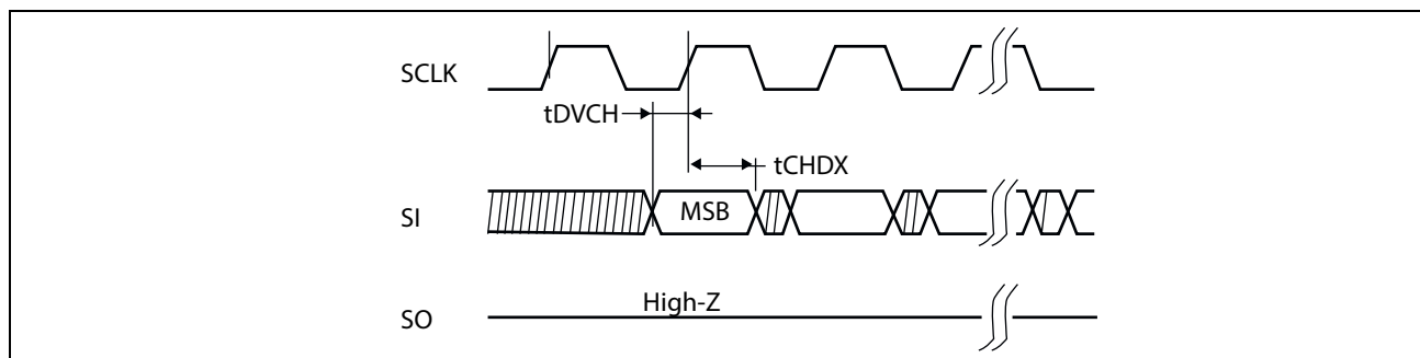
Figure 32. Input Timing
