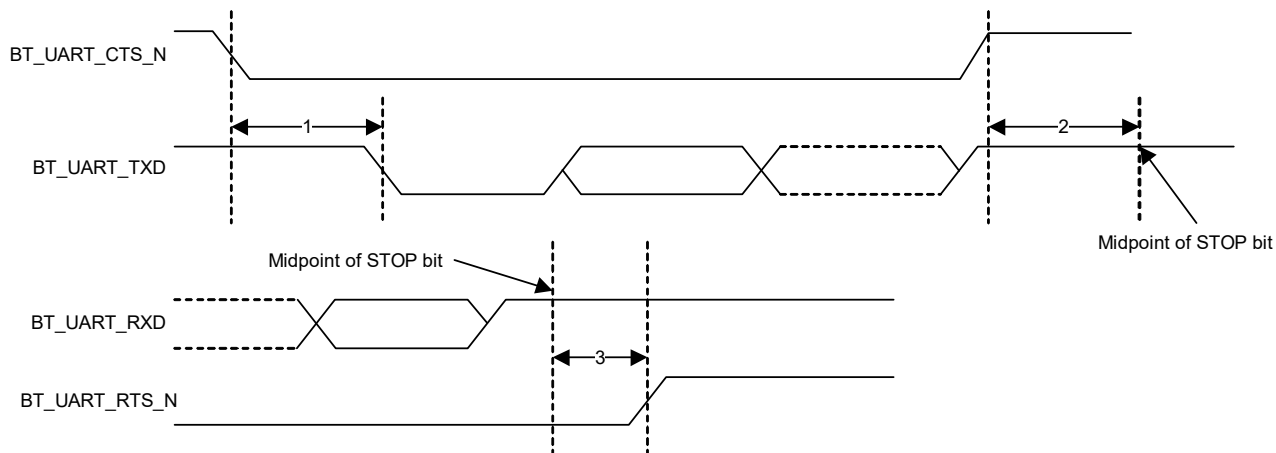
Figure 14. UART Timing
