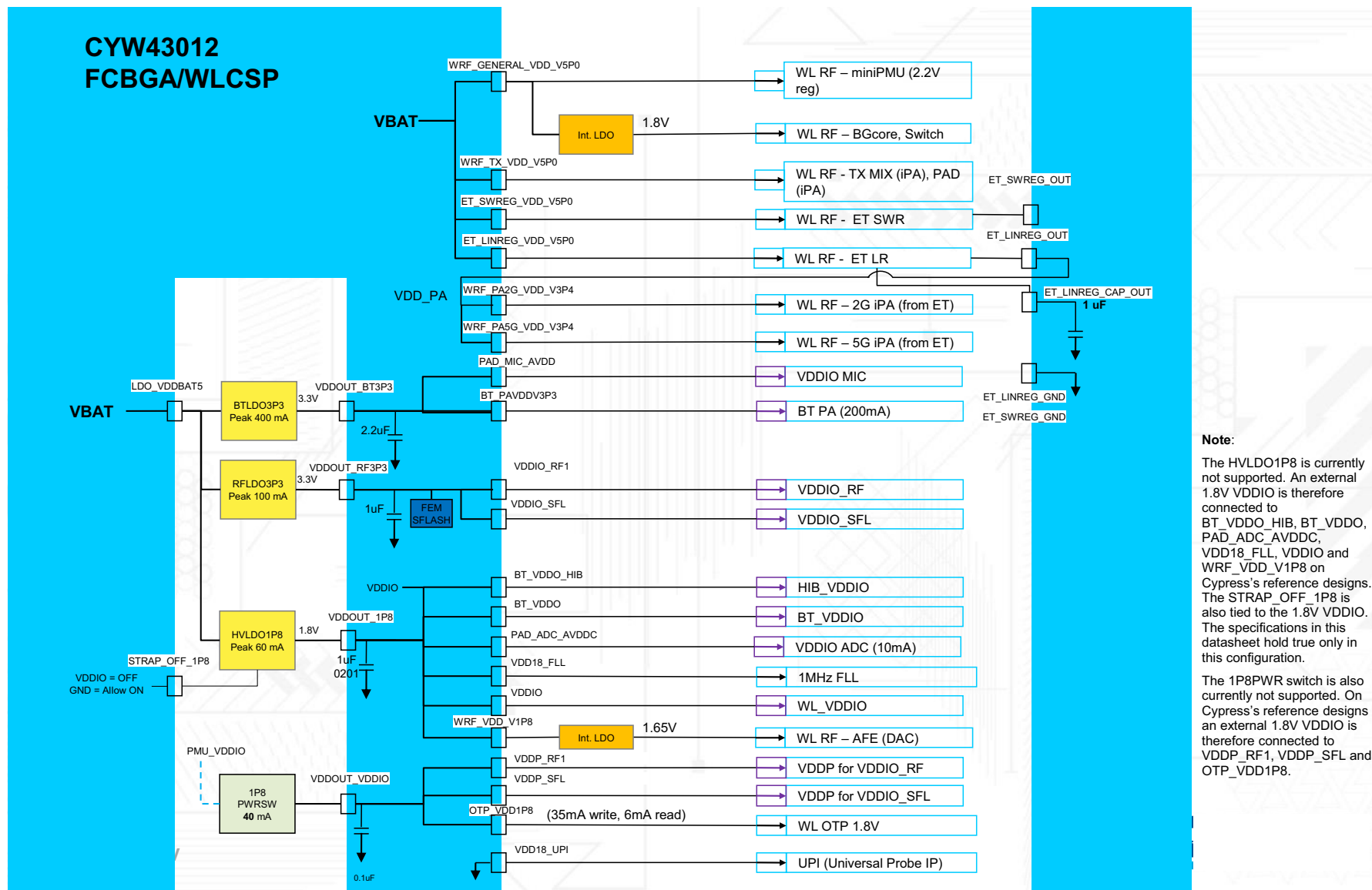
Figure 4. Typical Power Topology FCBGA/WLCSP (Page 2 of 2)
