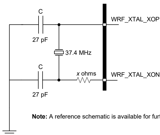
Figure 11. Recommended Oscillator Configuration
