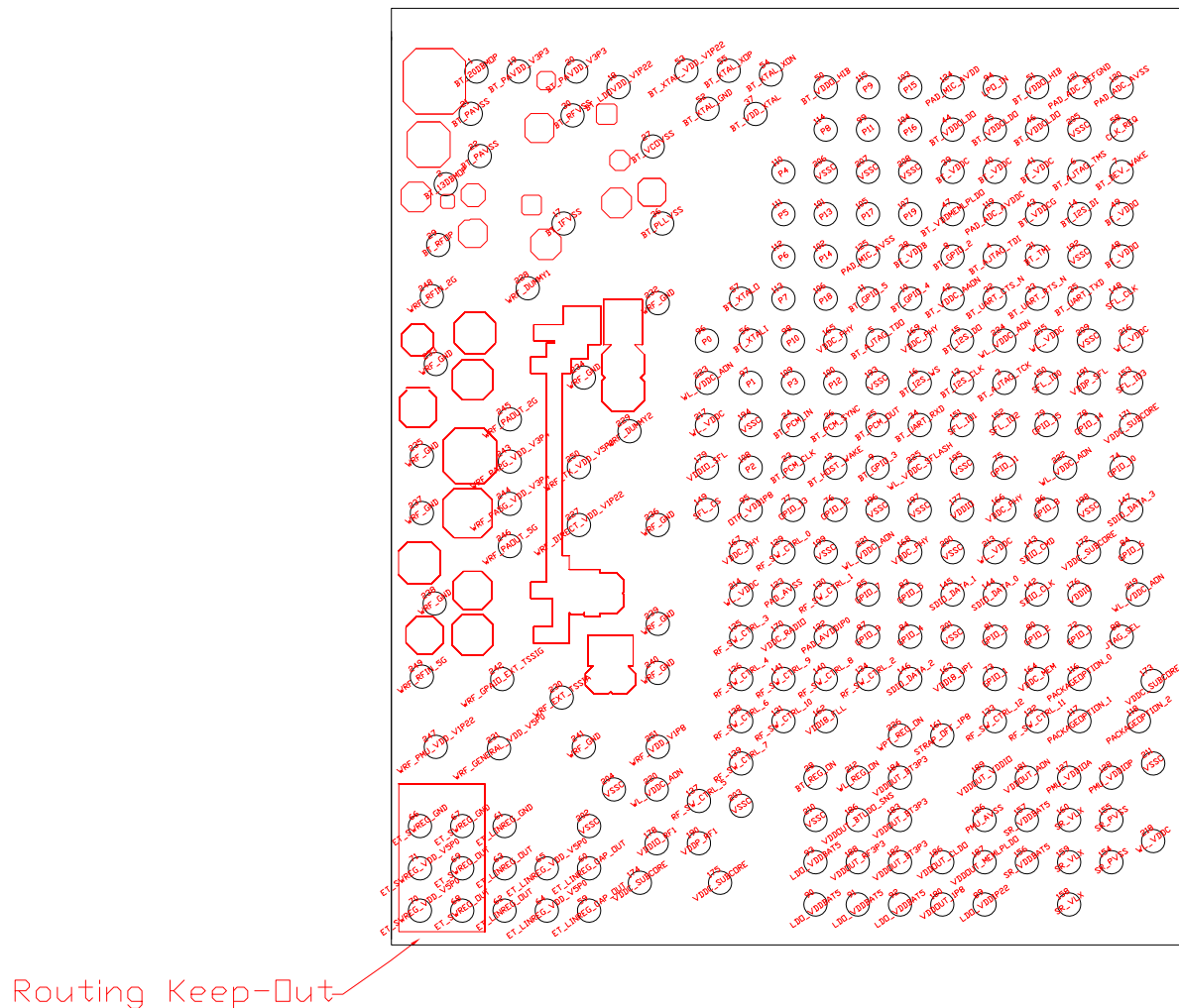
Figure 41. Keep-Out Areas (Package Top View, Bumps Facing Down)
