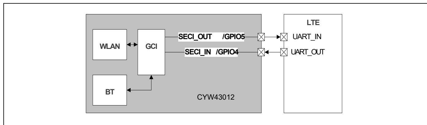
Figure 19. Cypress GCI or BT-SIG WCI-2 Coexistence Interface for Cypress BT/ZigBee radios or LTE radios
