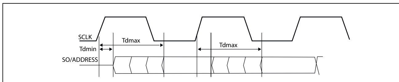
Figure 33. Output Timing
