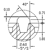
DETAIL "K" SCALE : 10/1
