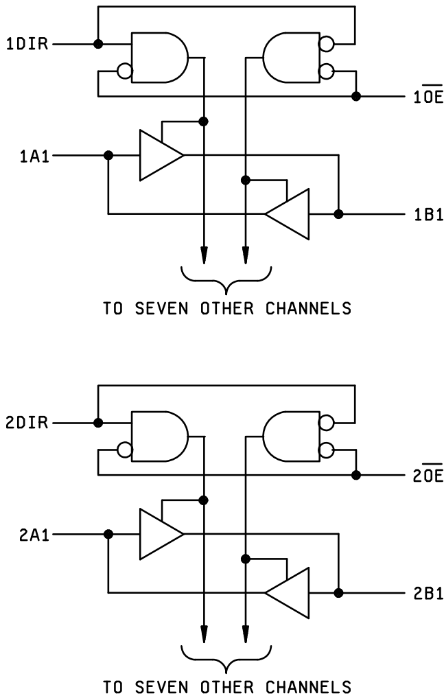
FIGURE 3. Logic diagram.
