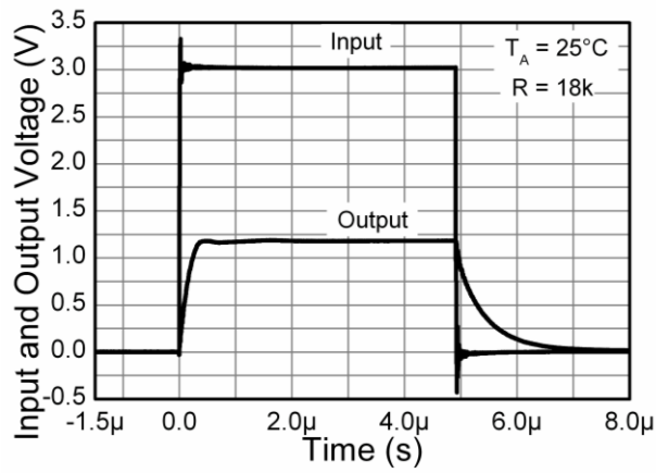
Pulse Response
