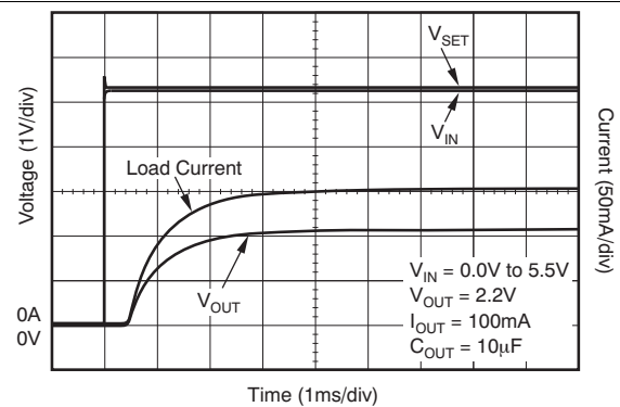
Figure 44. TPS780330220 Input Voltage vs Delay to Output
