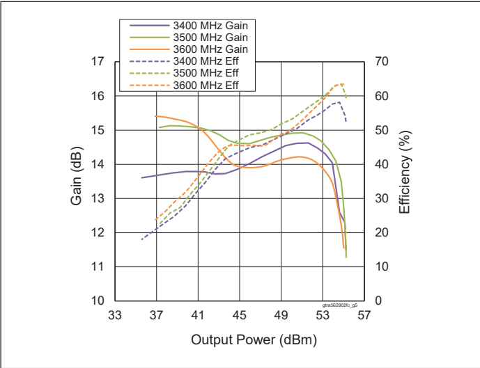
Figure 4. CW Performance
