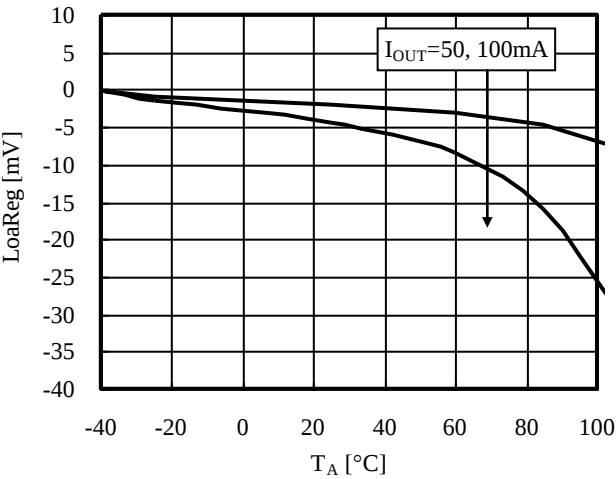
■ Load Regulation
