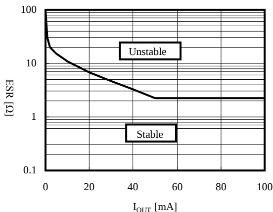
Figure 3. C_{\text{out}} = 0.47\mu\text{F}
