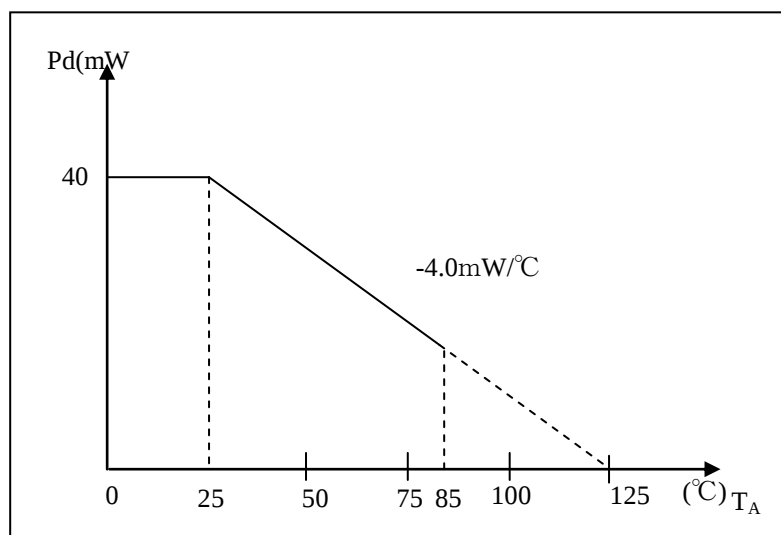
Figure 2. Maximum Power Dissipation
