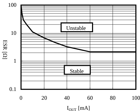
Figure 5. C_{\text{OUT}} = 1.0\mu\text{F}
