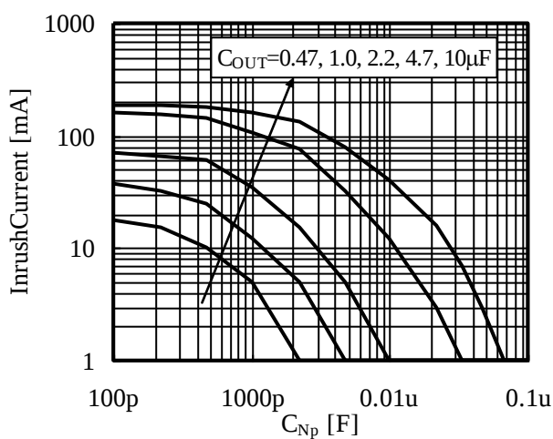
■ InRush Current vs C_{\text{NP}}
