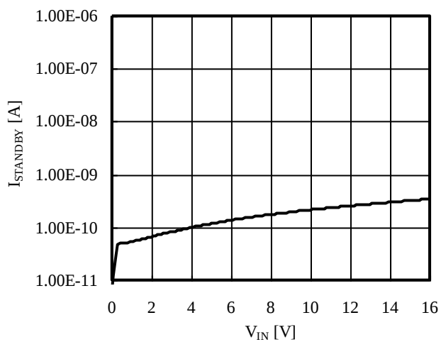
■ Standby Current ( V_{\text{CONT}}=0\text{V} )
