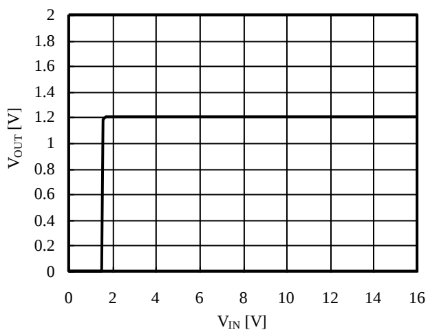
■ Line Regulation
