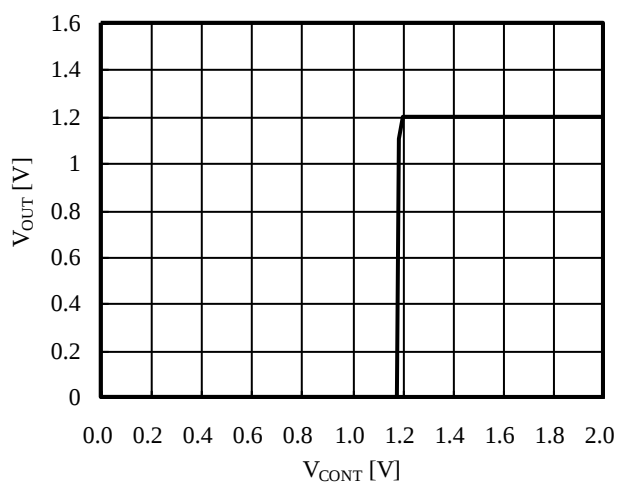
■ VOUT ON/OFF Point
