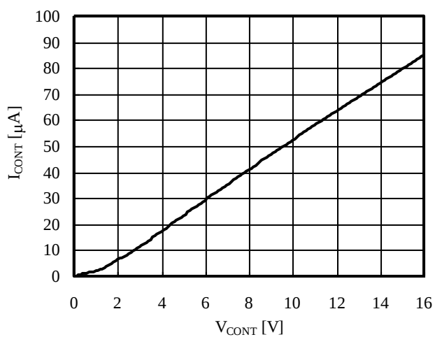
■ Control Current
