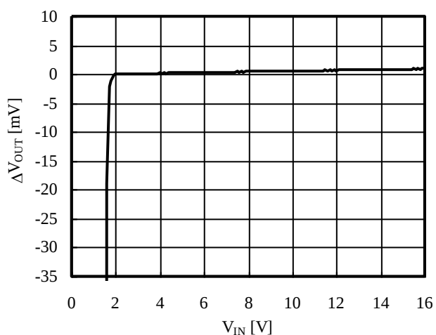
■ Line Regulation
