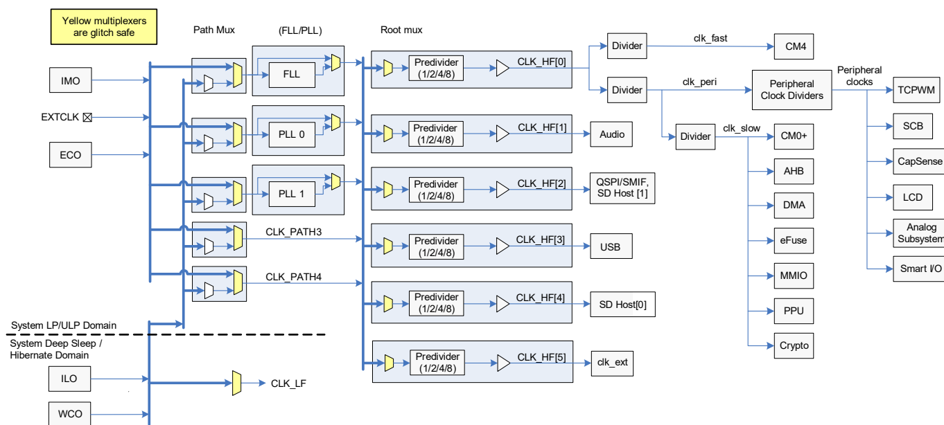
Figure 3. Clocking Diagram
