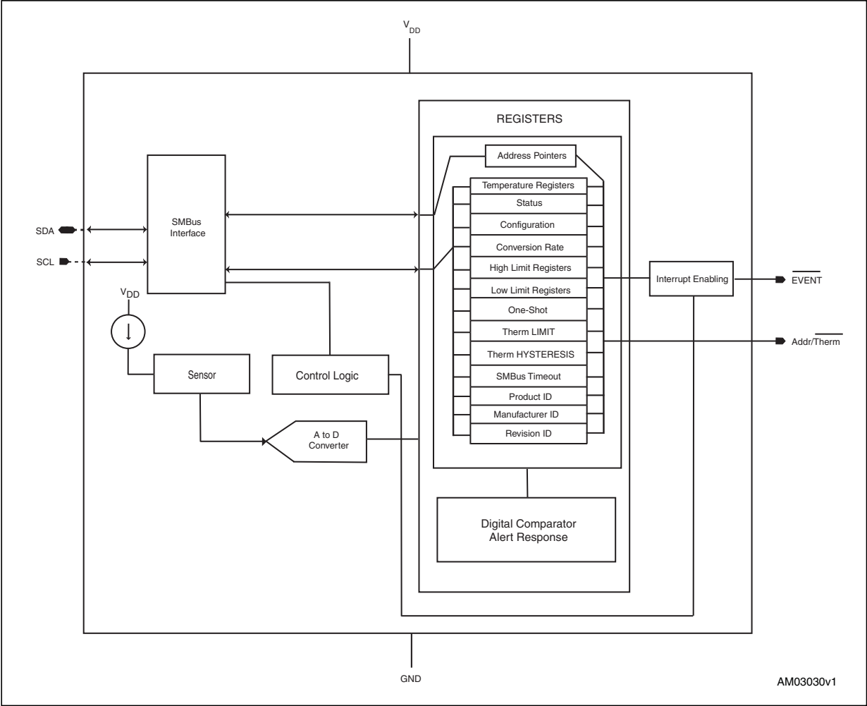
Figure 3. Block diagram
