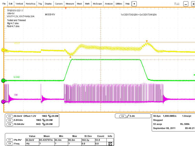
Figure 11. Load Transient
