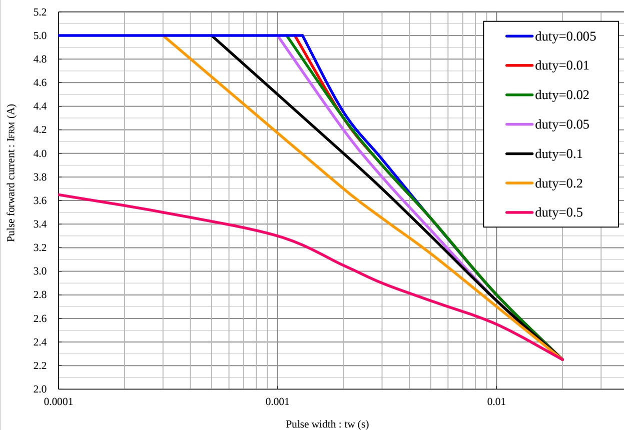
Maximum ratings of pulse forward current
