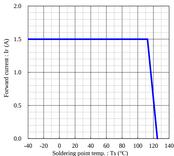
Maximum ratings of forward current
