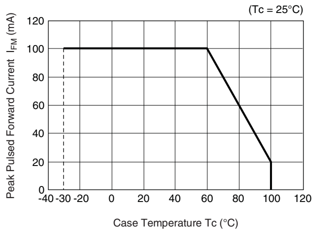
Fig. 3 Peak Pulsed Forward Current vs. Case Temperature
