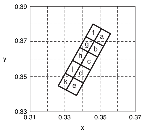
Fig. 8 Chromaticity Diagram
