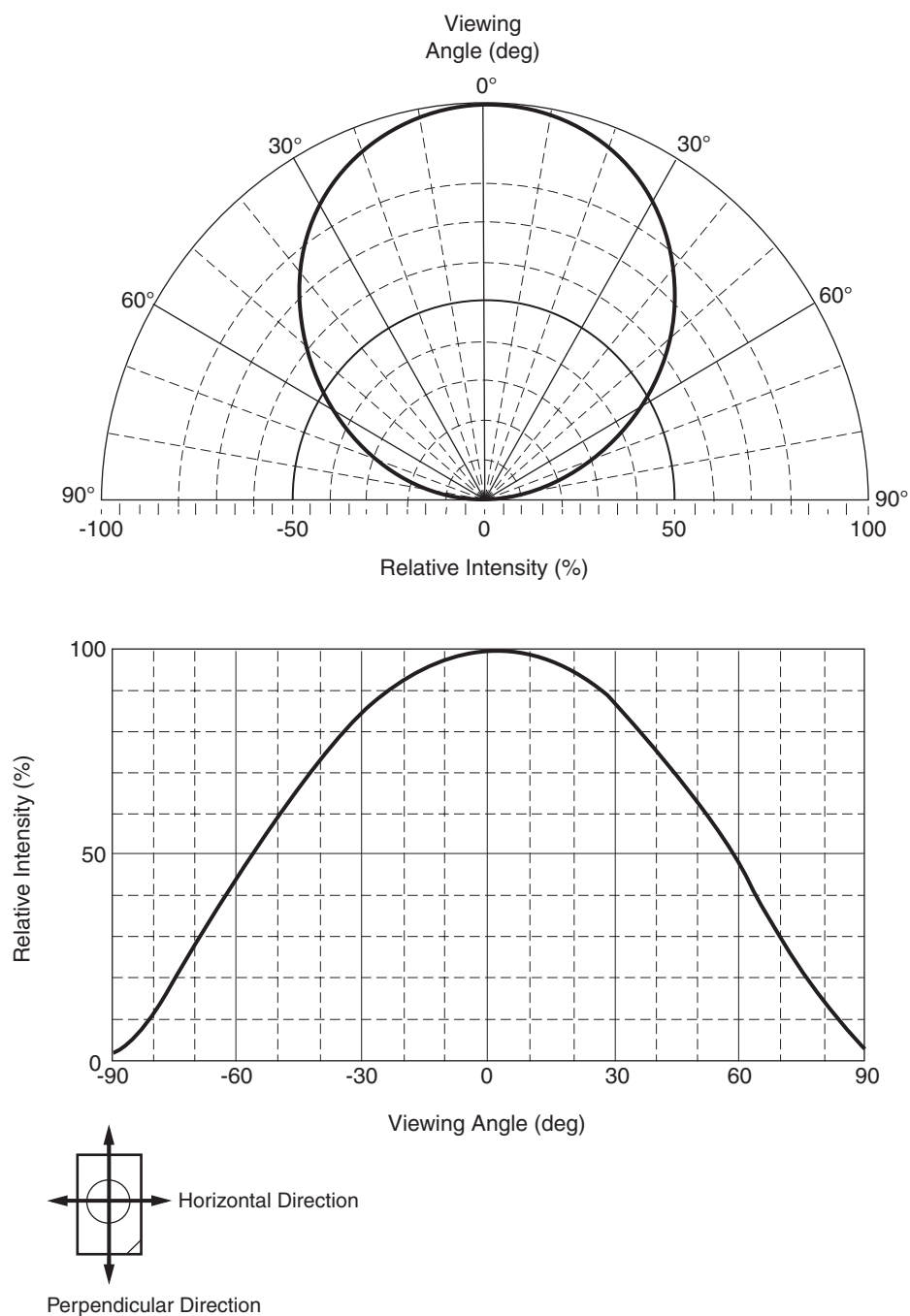
Fig. 7 Radiation Pattern
