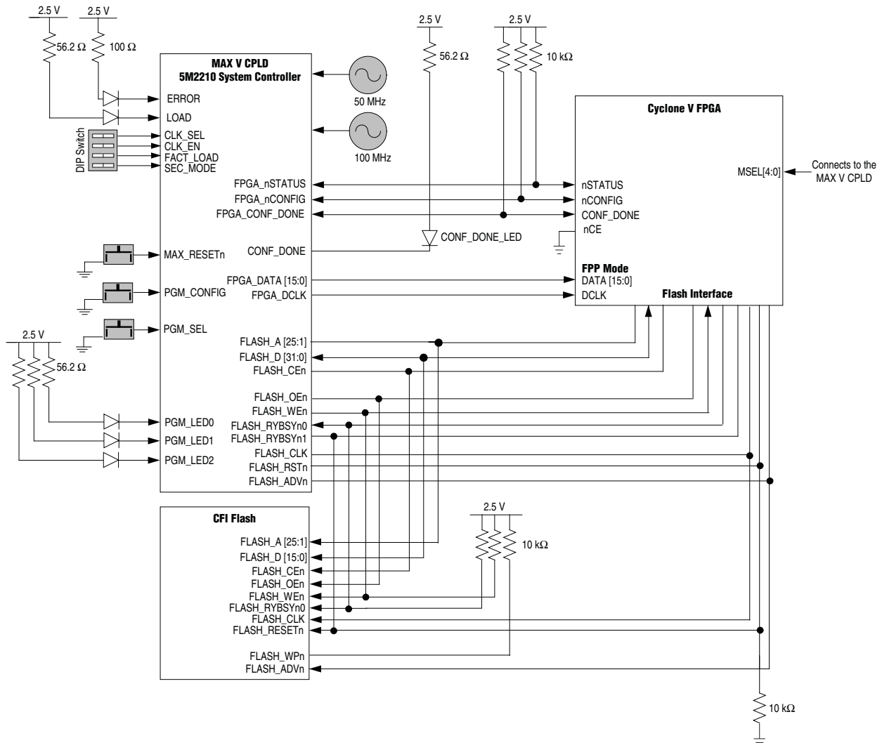
Figure 2-4. PFL Configuration
