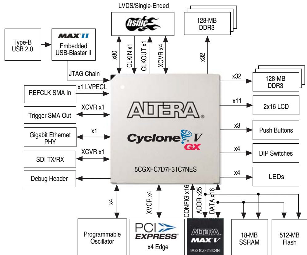
Figure 1-1. Cyclone V GX FPGA Development Board Block Diagram
