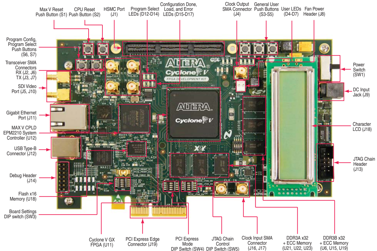
Figure 2–1. Overview of the Cyclone V GX FPGA Development Board Features
