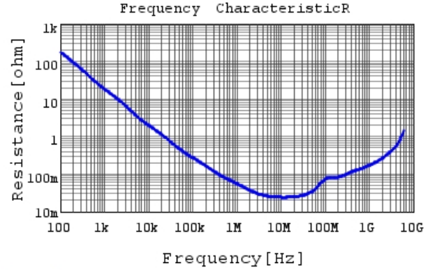
GRM155R61C473KA01 R DCOV, 25degC
