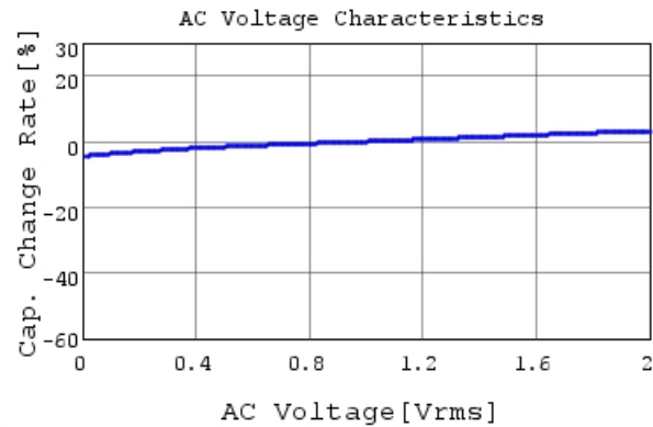
GRM155R61C473KA01 C-AC Voltage capchange, Dc
