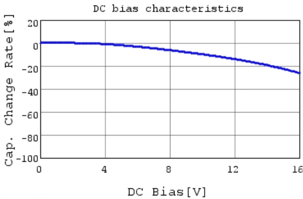
GRM155R61C473KA01 C-DC bias capchange, 25.0c
