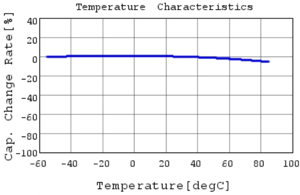
GRM155R61C473KA01 C-Temp. capchange, DC0.0V,
