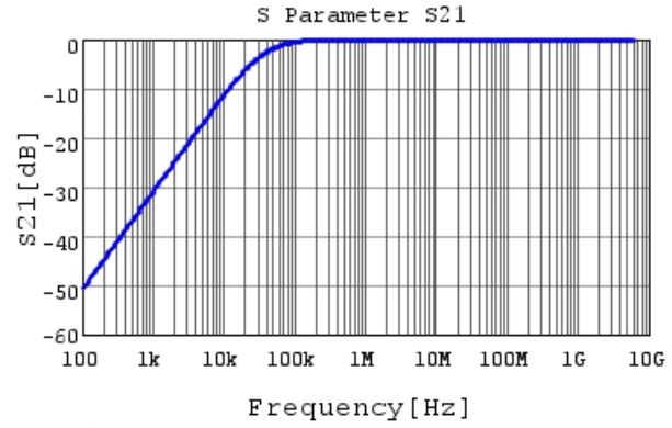
GRM155R61C473KA01 S21 DC0V,25degC
