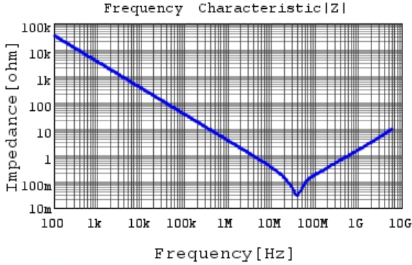
GRM155R61C473KA01 |Z| DCOV, 25degC
