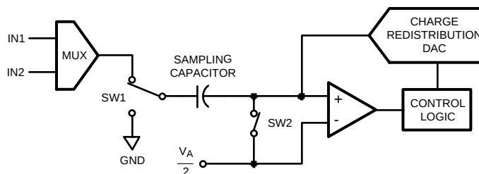
Figure 50. ADC122S101 in Hold Mode
