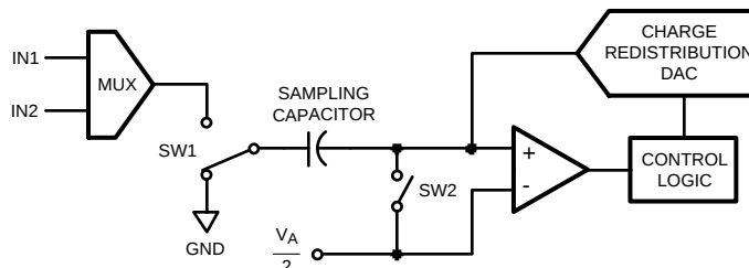
Figure 50. ADC122S101 in Hold Mode
