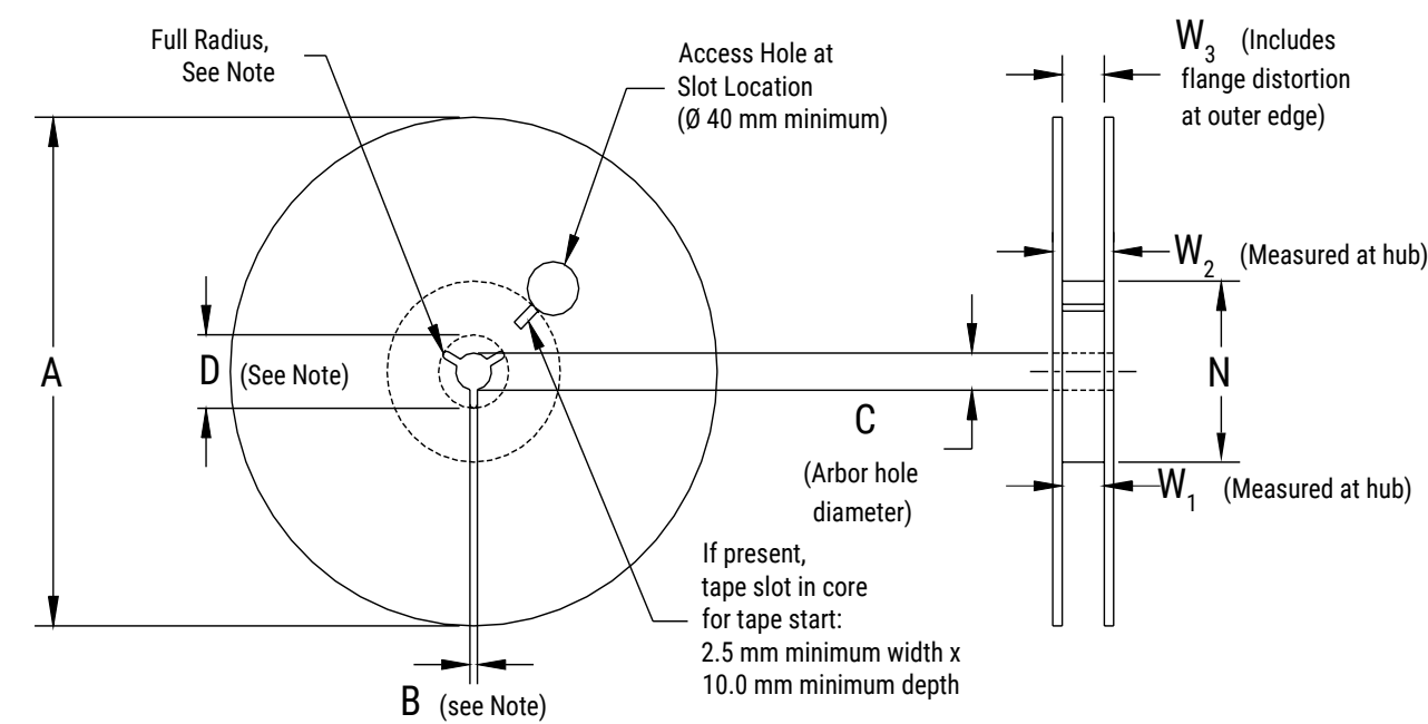
Figure 6 – Reel Dimensions
