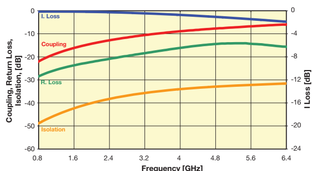
CP0402PxxxxBNTR
