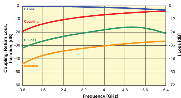
CP0402PxxxxANTR
