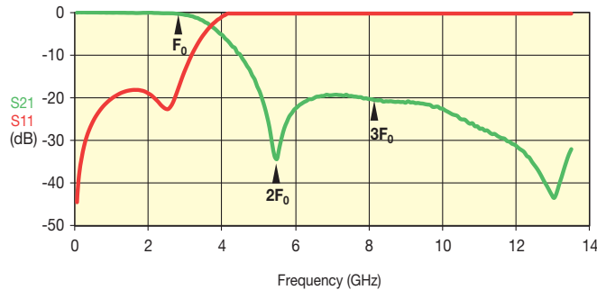
LP0402N2690ANTR
