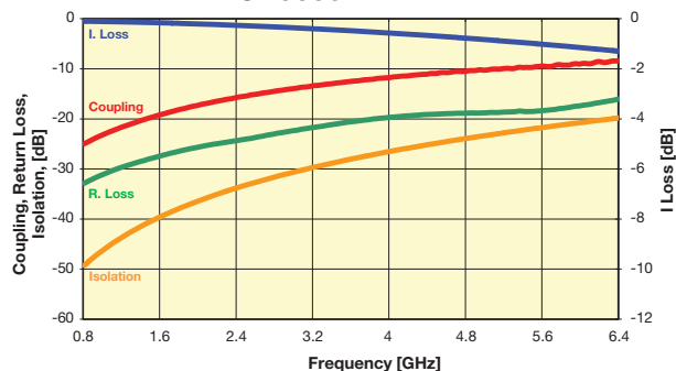
CP0603AxxxxMNTR
