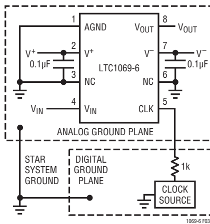
Figure 3. Connections for Dual Supply Operation
