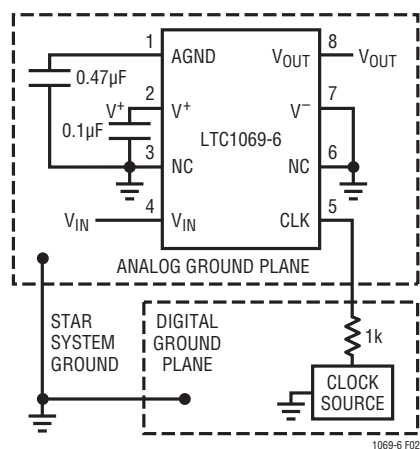
Figure 2. Connections for Single Supply Operation
