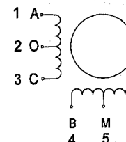
Wiring Diagram
