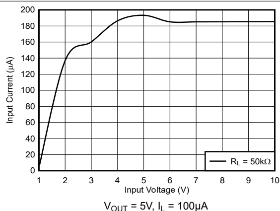
Figure 5-5. Input Current vs Input Voltage (Legacy Chip)
