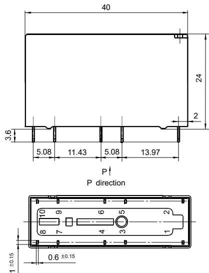
Outline Dimensions
