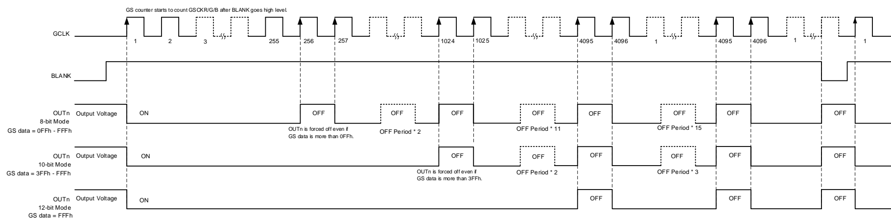
Figure 13. 8-, 10-, 12-Bit Mode PWM Counter With Auto-Repeat Mode
