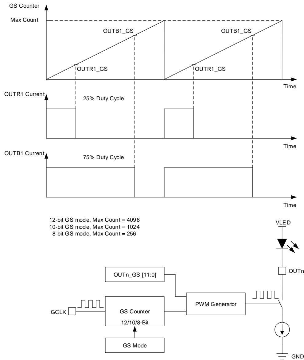
Figure 22. PWM Generator
