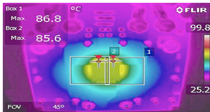
Figure 14. Thermal Image 12V to 5V, 50A with 200LFM Airflow without Heat Sink
