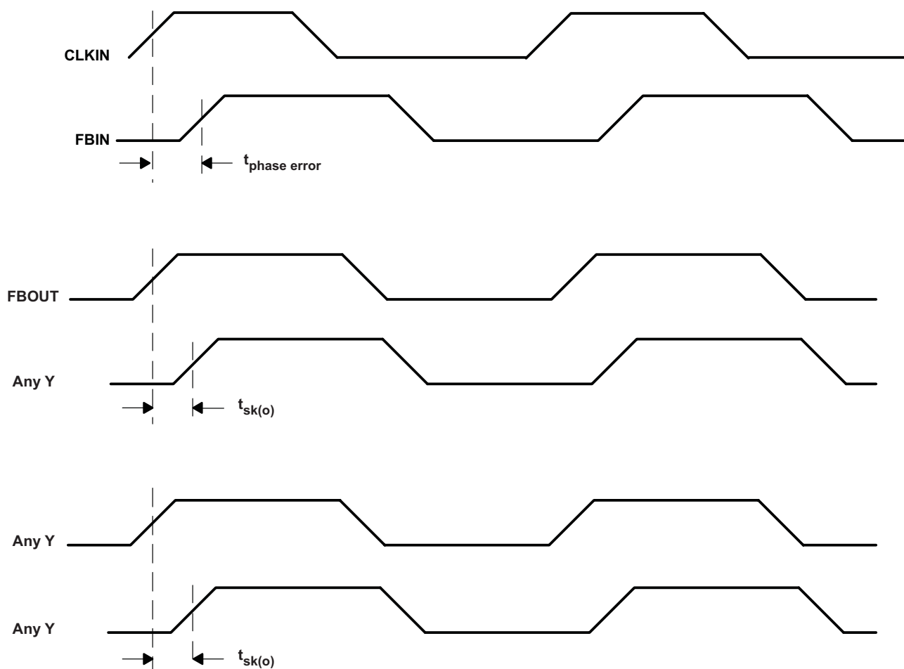
Figure 2. Skew Calculations
