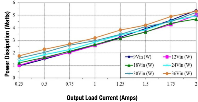
24QS24.50SBM Power Dissipation vs. Line and Load
