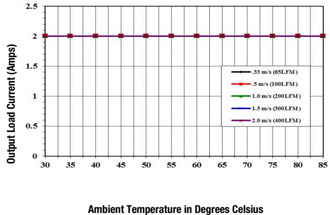
24QS24.50SBM Temperature Derating Vin 12V (air flow from Pin 1 to Pin 3 on PCB)
