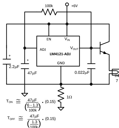
Figure 45. Flasher Circuit
