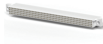
4 Row AMP-HDI Receptacle Assembly
