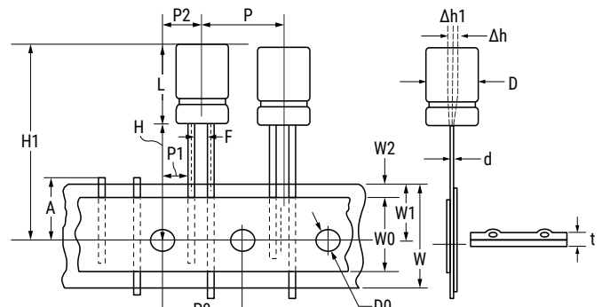
Fig. 4 (Diameter for \Phi 10 ) 10 mm EA
