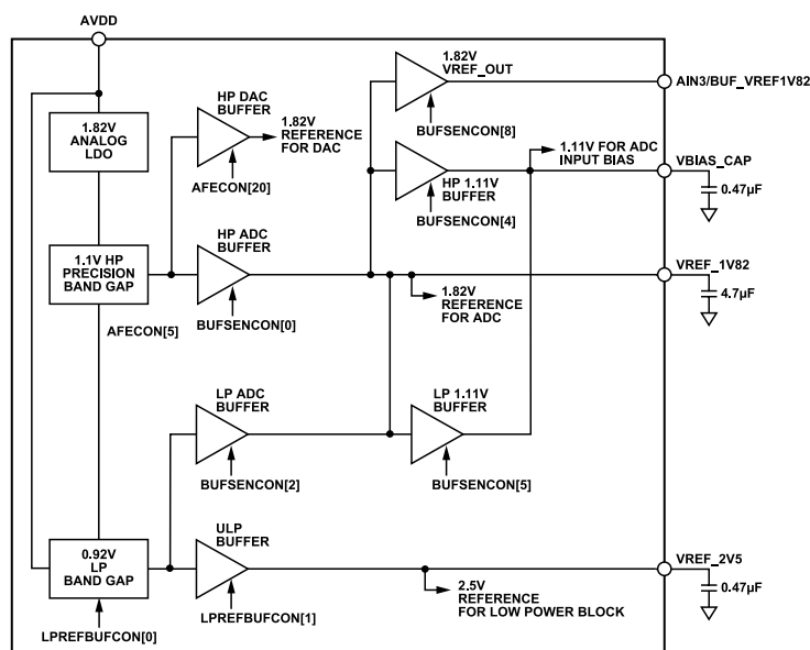
Figure 37. Precision Voltage References
