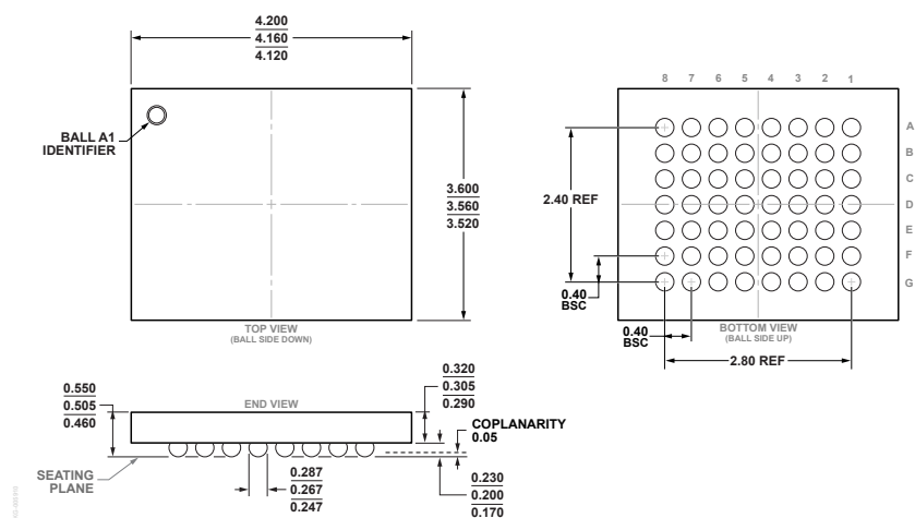
Figure 58. 56-Ball Wafer Level Chip Scale Package [WLCSP] (CB-56-3)
