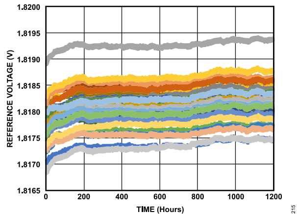
Figure 15. V_{REF} 1.8 V Lifetime Drift
