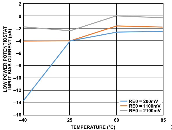
Figure 13. Low Power Potentiostat Input Bias Current vs. Temperature
