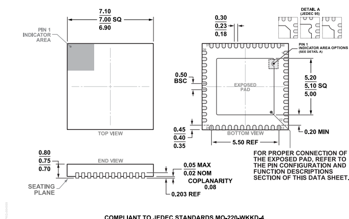
Figure 59. 48-Lead Lead Frame Chip Scale Package [LFCSP] 7 mm × 7 mm Body and 0.75 mm Package Height (CP-48-4)
