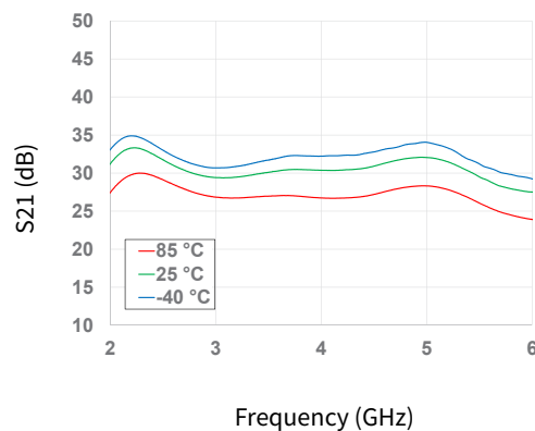
Figure 35. Gain vs Frequency as a Function of Temperature
