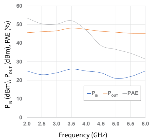
Figure 47. Output Power and Power Added Eff. vs Frequency when Optimized for Mamimum Output Power
