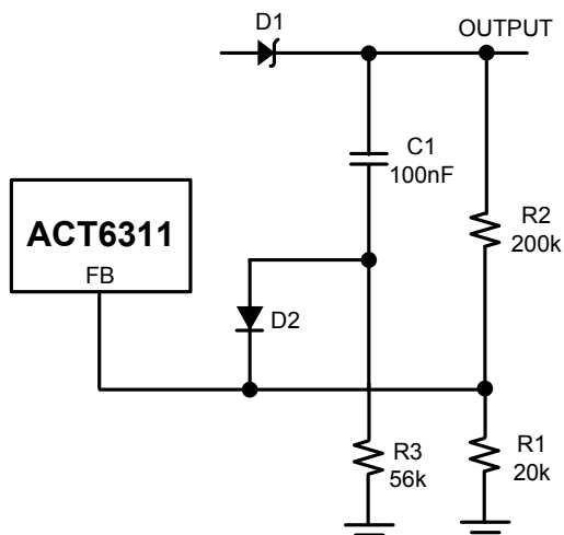
Figure 8: Soft-Start Circuit
