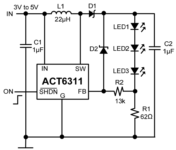
Figure 9: Open-Circuit Protection
