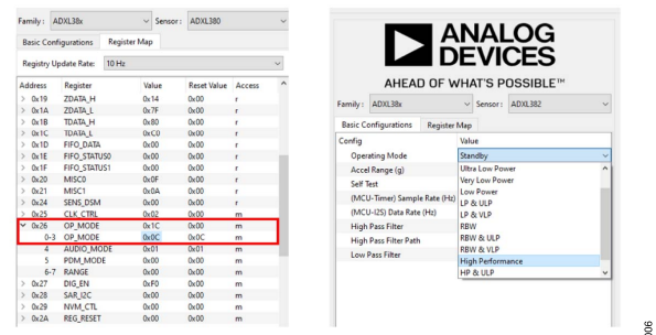
Figure 6. Operation Mode (High Performance)
