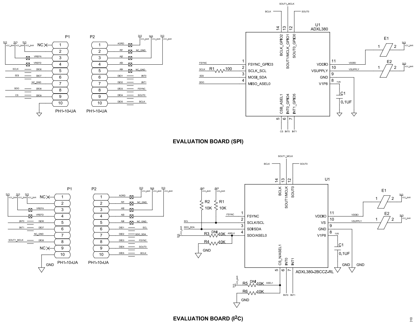
Figure 10. EVAL-ADXL380-EB-1Z or EVAL-ADXL380-EB-2Z Evaluation Board Schematic
