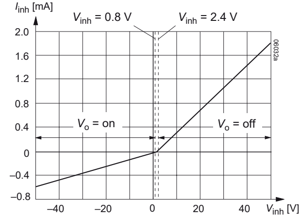
Fig. 15 Typical inhibit current I_{inh} versus inhibit voltage V_{inh}
