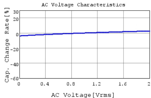
GRJ31CR71H475ME11 C-AC Voltage capchange, D
