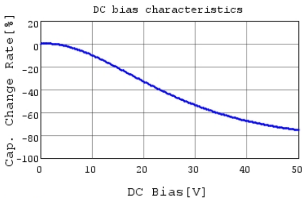
GRJ31CR71H475ME11 C-DC bias capchange, 25.0C
