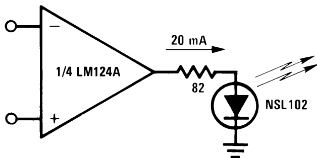
Figure 17. DC Summing Amplifier ( V_{\text{IN}}\text{'S} \geq 0\text{ V}_{\text{DC}} And V_0 \geq V_{\text{DC}} )
