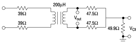
Figure 22. Test Load C
