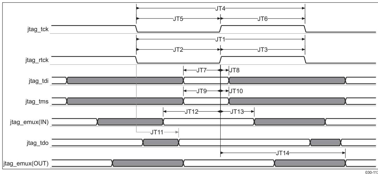
Figure 6-73. JTAG Interface Timing Free Running Clock Mode
