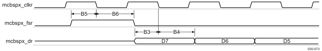
Figure 6-42. McBSP Falling Edge Receive Timing in Slave Mode
