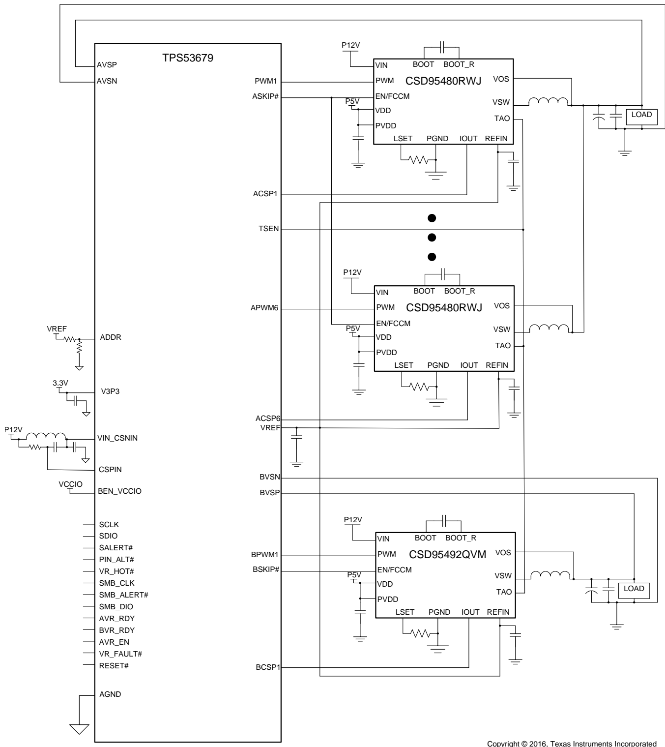
Figure 1. Application Schematic
