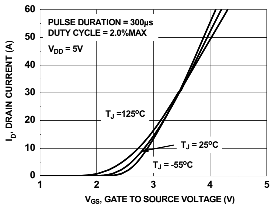
Figure 16. Transfer Characteristics
