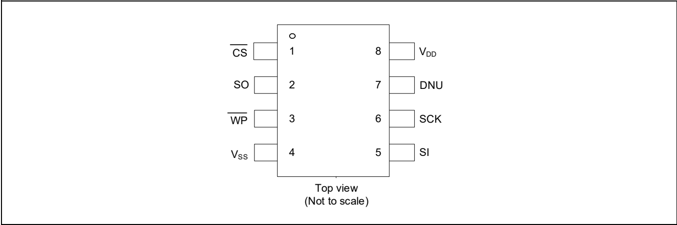
Figure 1 8-pin SOIC pinout
