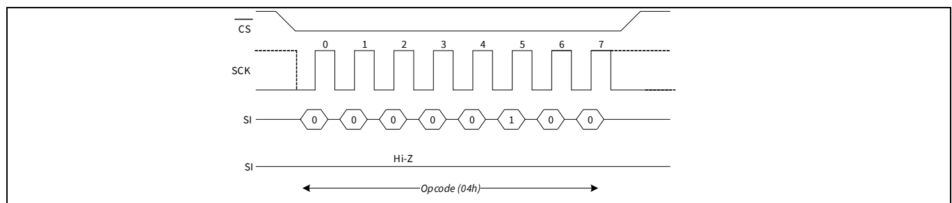
Figure 7 WRDI bus configuration
