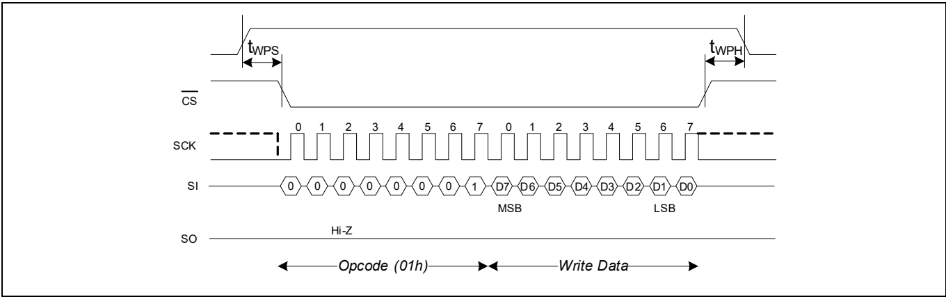
Figure 23 Write protect timing during write status register (WSR) operation
