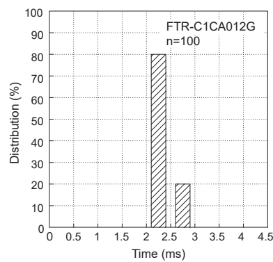
Pulse characteristics
