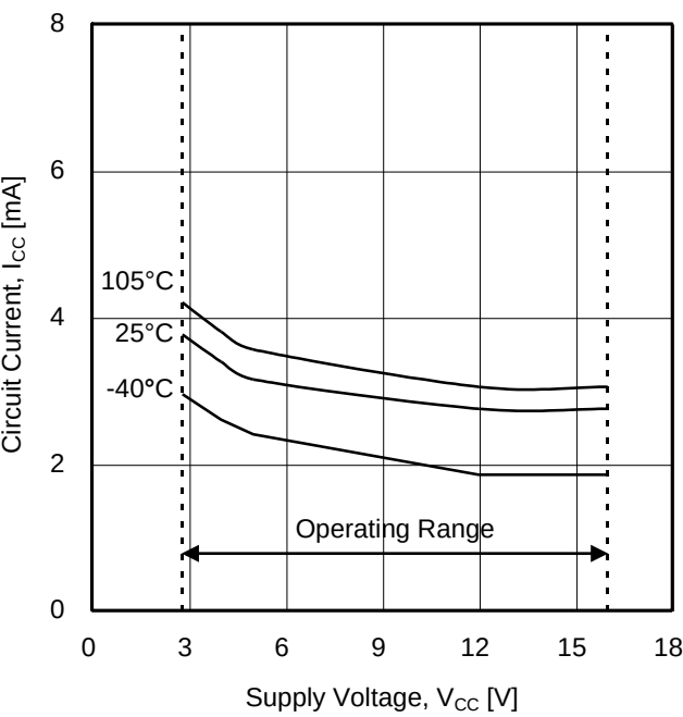
Figure 1. Circuit Current
