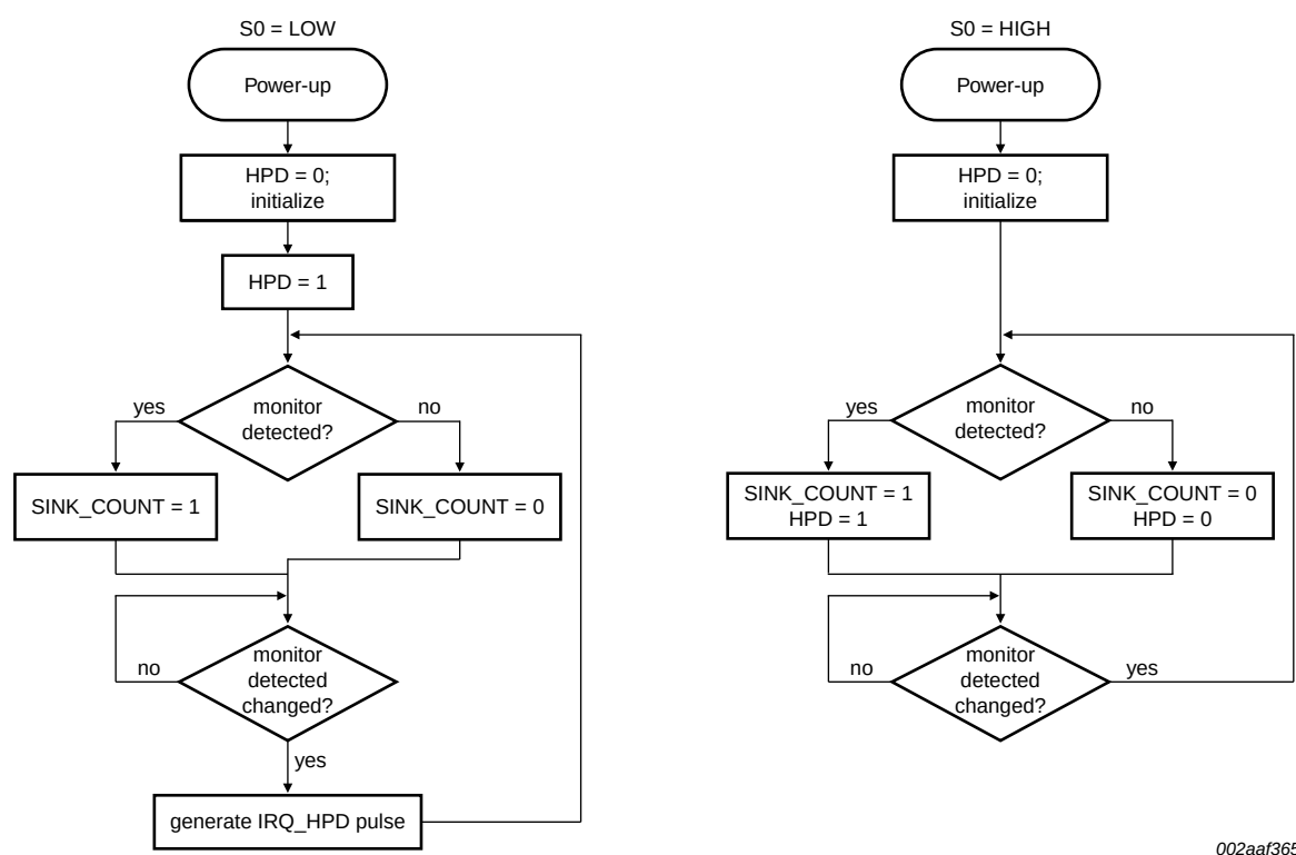
Fig 3. Pin S0 behavior
