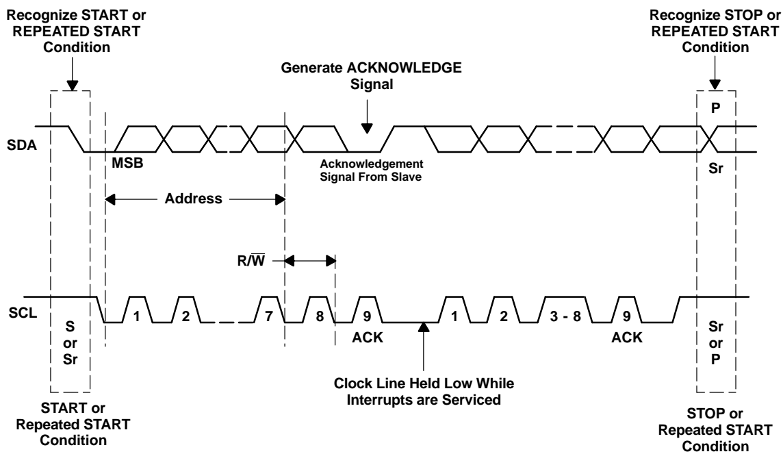
Figure 50. Bus Protocol
