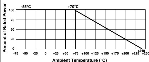
Figure 1 – Typical Power Derating Curve
