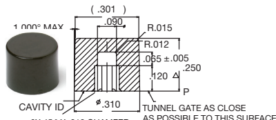
Cap, .120" DIA. Plungers
