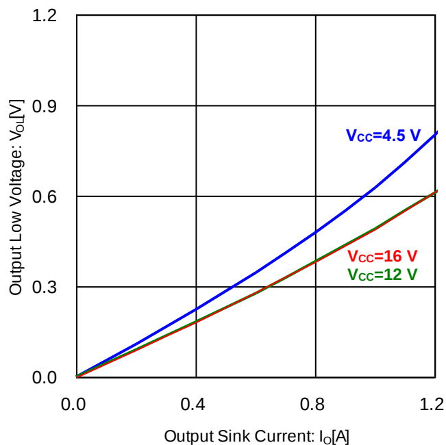
Figure 5. Output Low Voltage vs Output Sink Current ( T_a=25\text{ }^{\circ}\text{C} )
