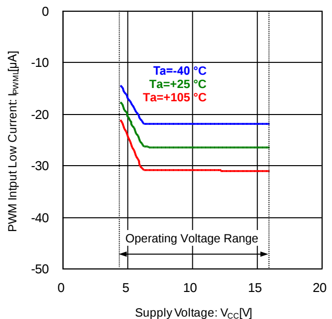
Figure 8. PWM Input Low Current vs Supply Voltage ( V_{\text{PWM}}=0\text{ V} )
