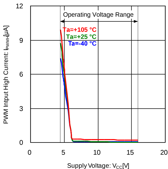
Figure 7. PWM Input High Current vs Supply Voltage ( V_{\text{PWM}}=5\text{ V} )
