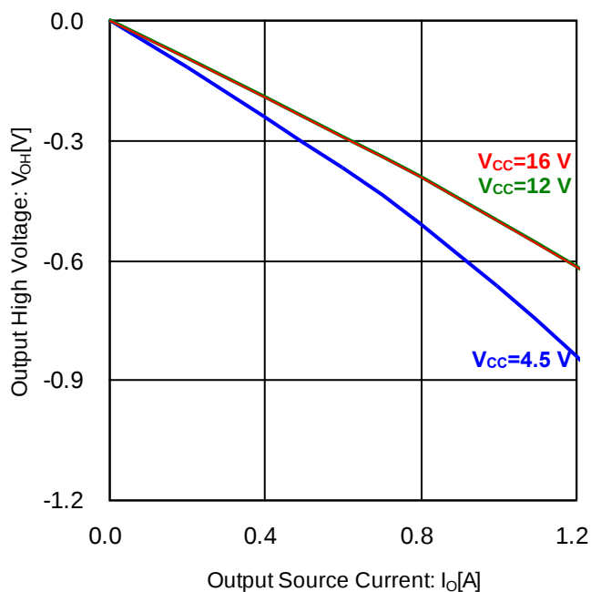
Figure 3. Output High Voltage vs Output Source Current ( T_a=25\text{ }^{\circ}\text{C} )
