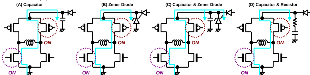
Figure 30. Measure Against V CC and Motor Driving Outputs Voltage
