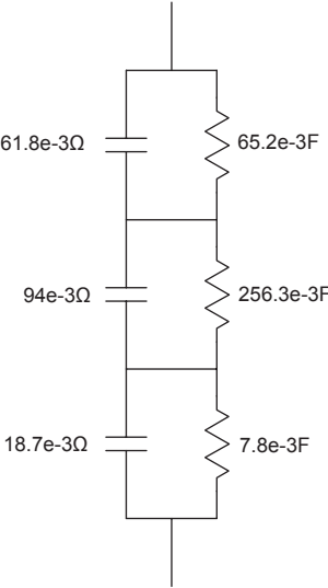
Figure 3a, Transient Thermal Impedance Model
