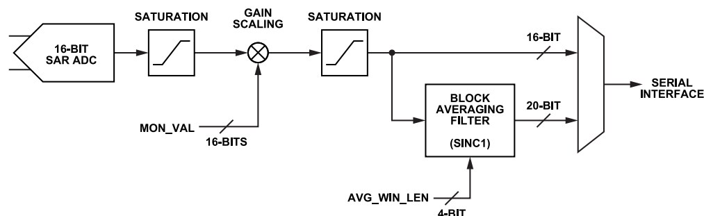
Figure 40. AD4052 Digital Processing Functionality
