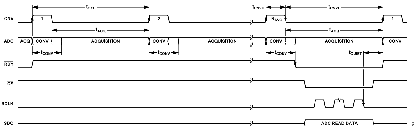
Figure 51. Averaging Mode Timing Diagram
