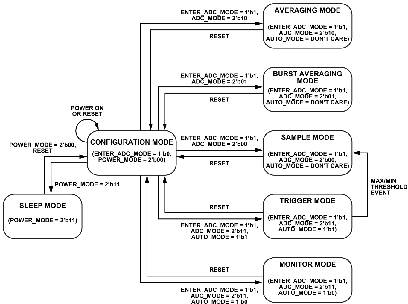
Figure 47. AD4052 State Machine Diagram
