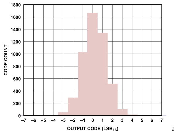
Figure 9. Histogram, Sample Mode (No Averaging)
