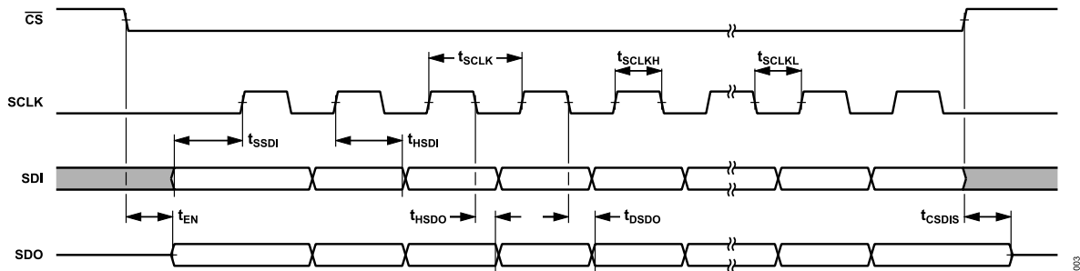
Figure 3. SPI Timing Specifications Diagram
