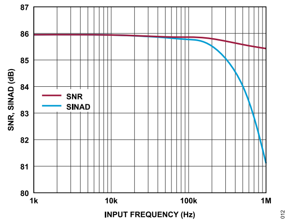
Figure 12. SNR, SINAD vs. Input Frequency
