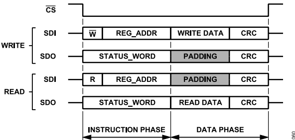
Figure 60. Configuration Mode SPI Format
