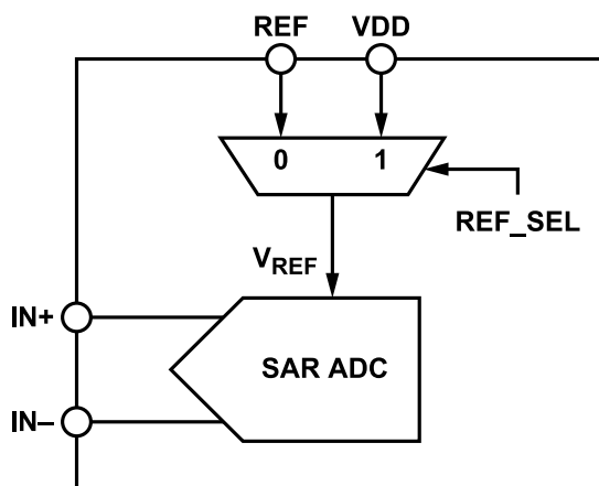
Figure 39. Reference Source Selection
