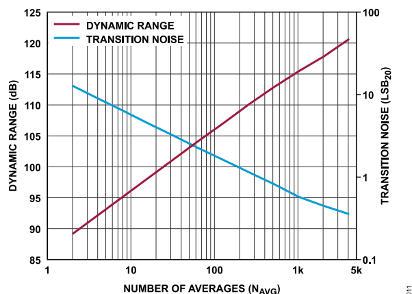
Figure 11. Dynamic Range and Transition Noise vs. N_{AVG}
