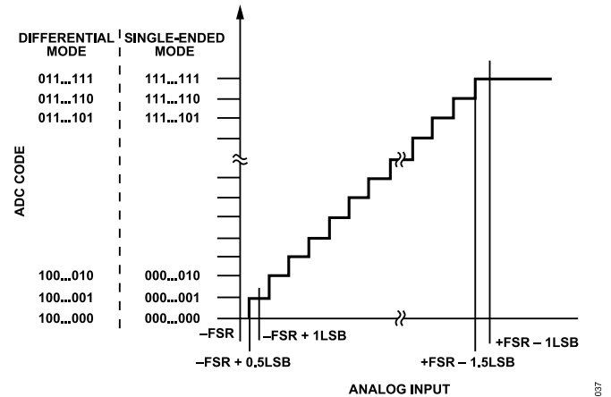
Figure 37. ADC Ideal Transfer Function
