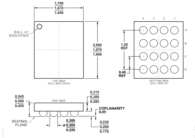
Figure 77. 16-Ball Wafer Level Chip Scale Package [WLCSP] (CB-16-26) Dimensions shown in millimeters
