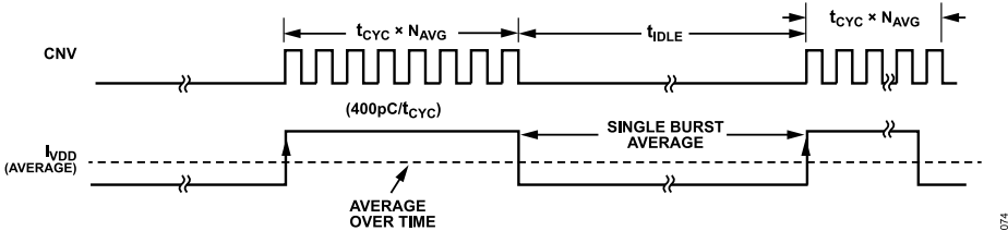
Figure 74. I_{DD} vs. Burst Conversions in Burst Averaging Mode
