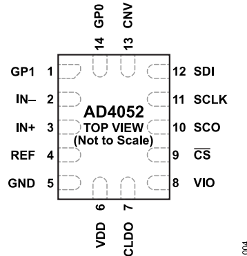
Figure 4. AD4052 LFCSP Pin Configuration
