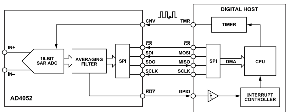
Figure 50. Averaging Mode Example Connection Diagram
