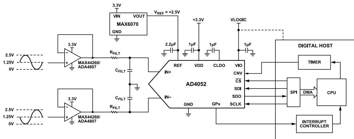
Figure 67. AD4052 Typical Application Diagram
