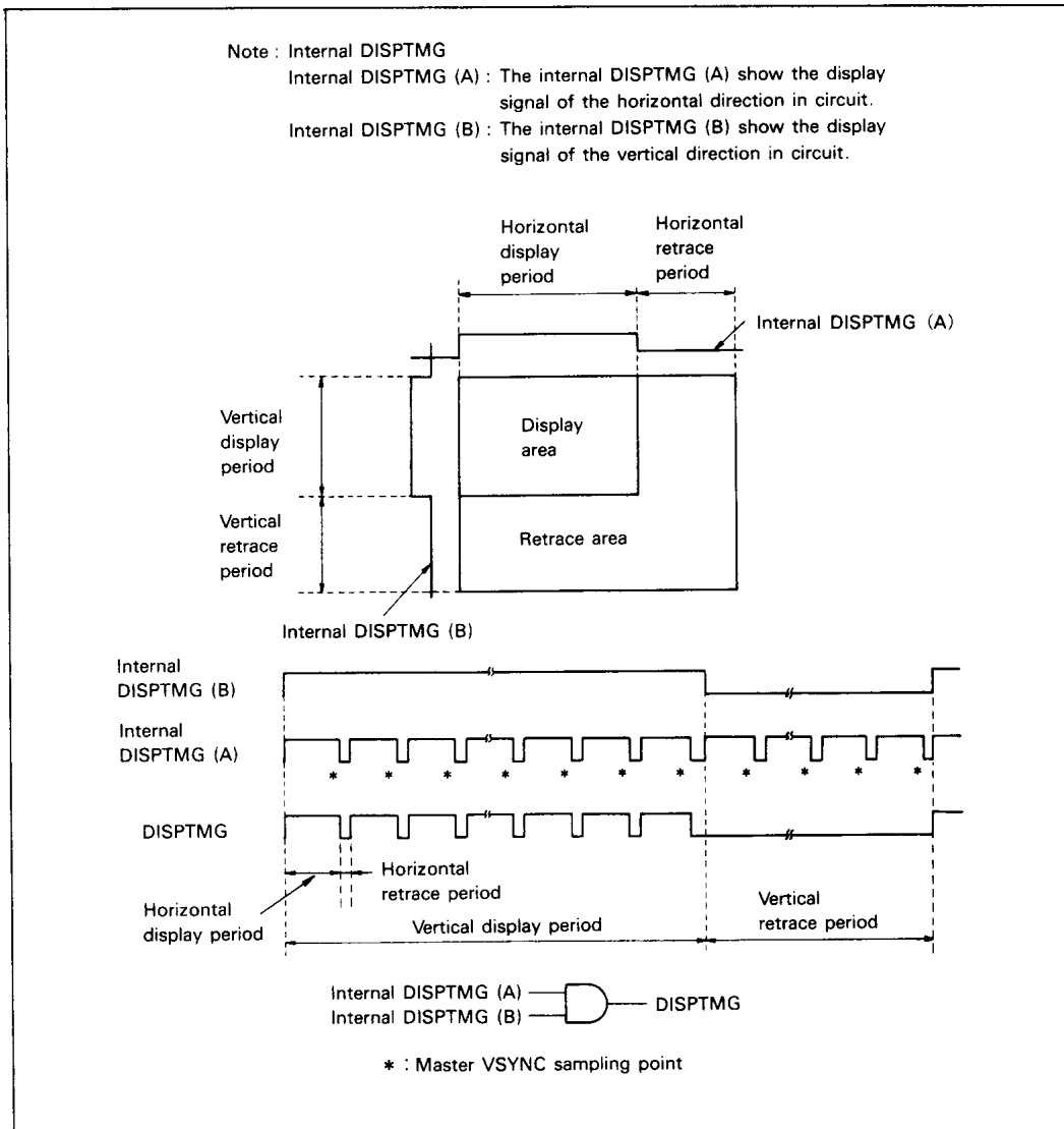
Figure 32-(b) External Sync Timing (TV Sync Mode: EXVSYNC)
