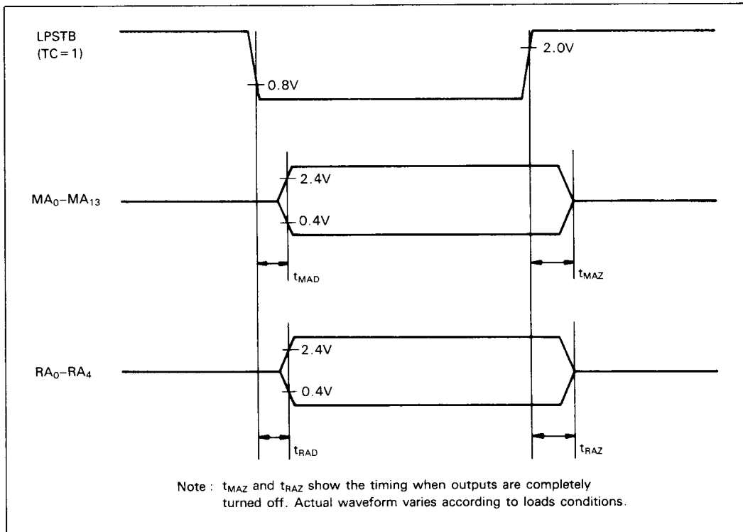
Figure 27 Three-State Delay Timing (Three-state mode: TC=1)
