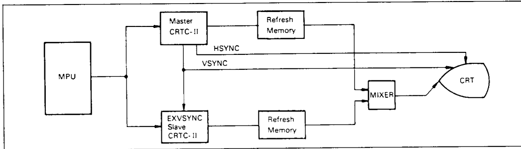
Figure 16 Master-Slave Mode
