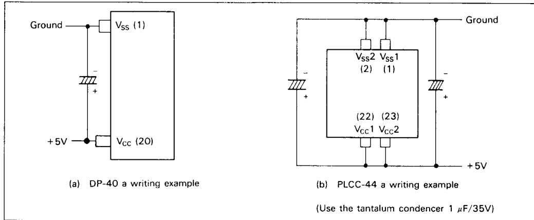
Figure 38 Note on Power Line Example
