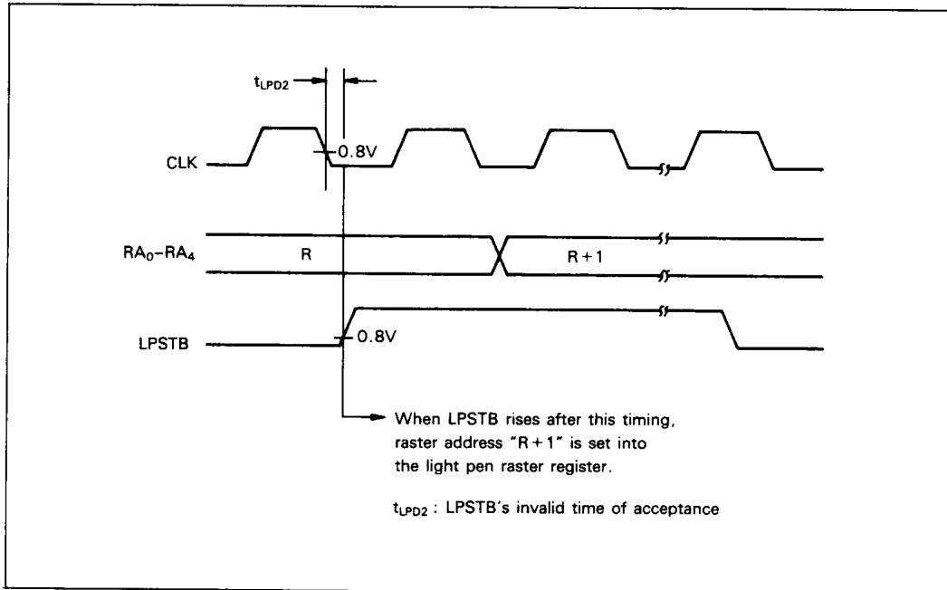
Figure 29 CRTC-II CLK, RA 0 -RA 4 and LPSTB Timing
