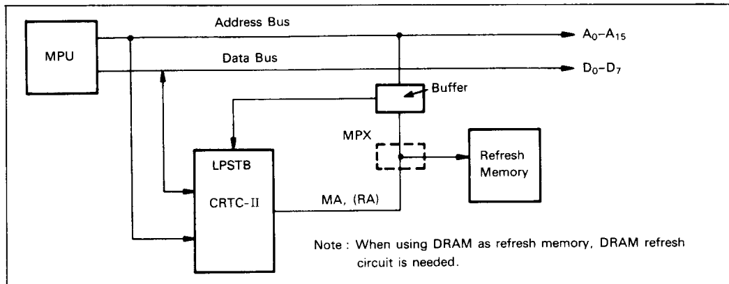
Figure 22 Three-State Control
