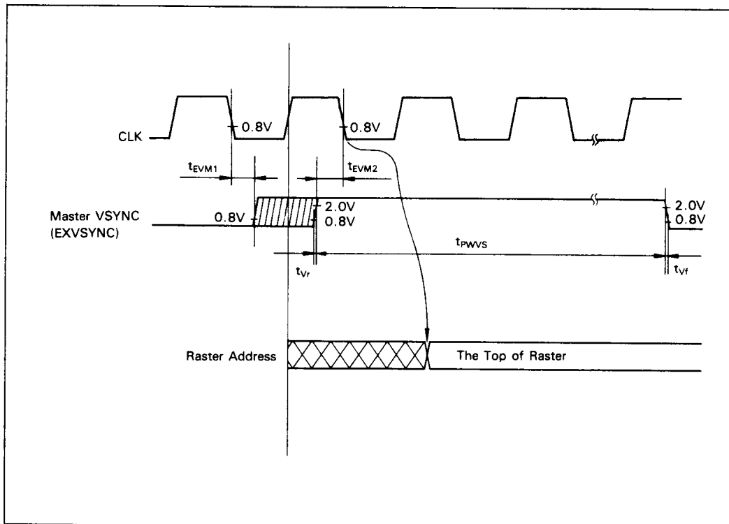
Figure 30 External Sync Timing (Master/Slave Mode)
