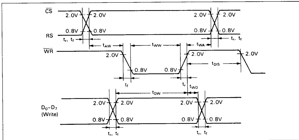
Figure 36 Write Sequence (HD6445)
