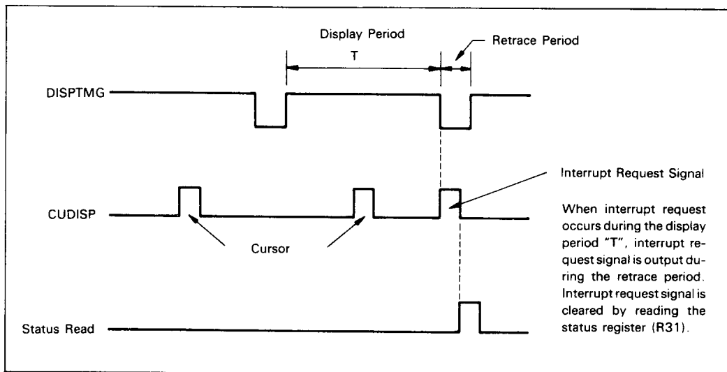
Figure 21 Interrupt Timing
