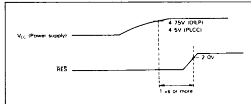
Figure 25 Reset at Power-on
