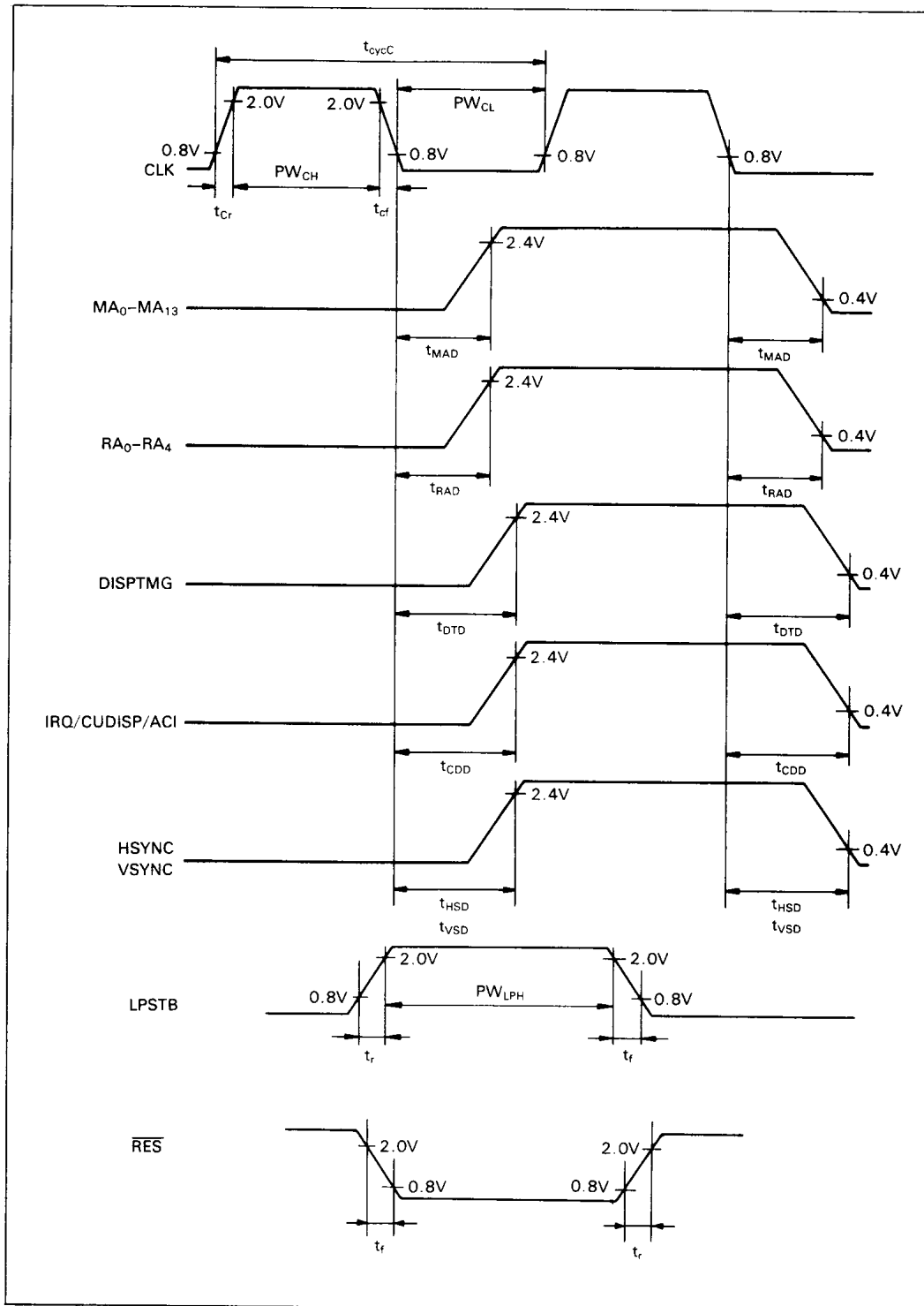
Figure 26 CRTC-II Timing Chart
