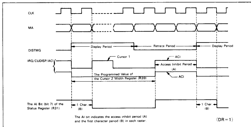
Figure 23 MPRAM Mode Output Timing
