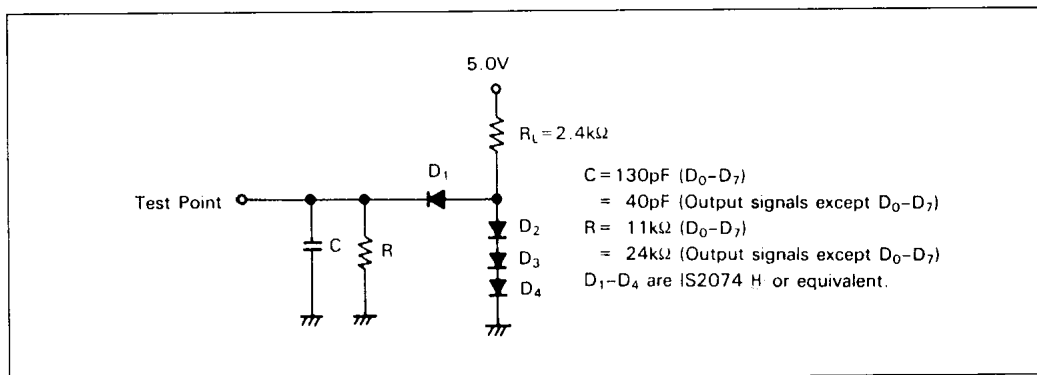
Figure 37 Test Load
