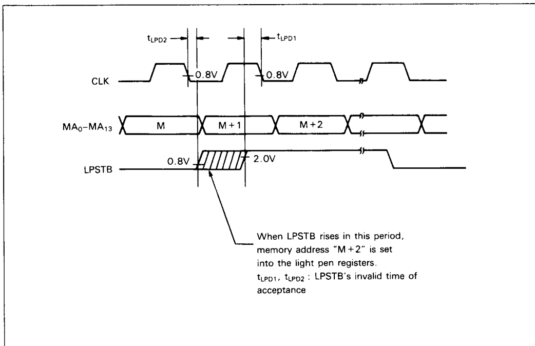
Figure 28 CRTC-II CLK, MA 0 -MA 13 , and LPSTB Timing
