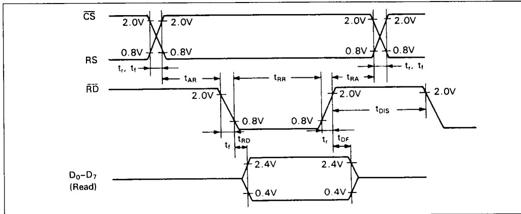
Figure 35 Read Sequence (HD6445)
