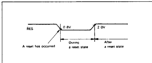
Figure 24 Reset Definition
